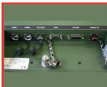
MOJAVE RD22 example for standard interfaces
